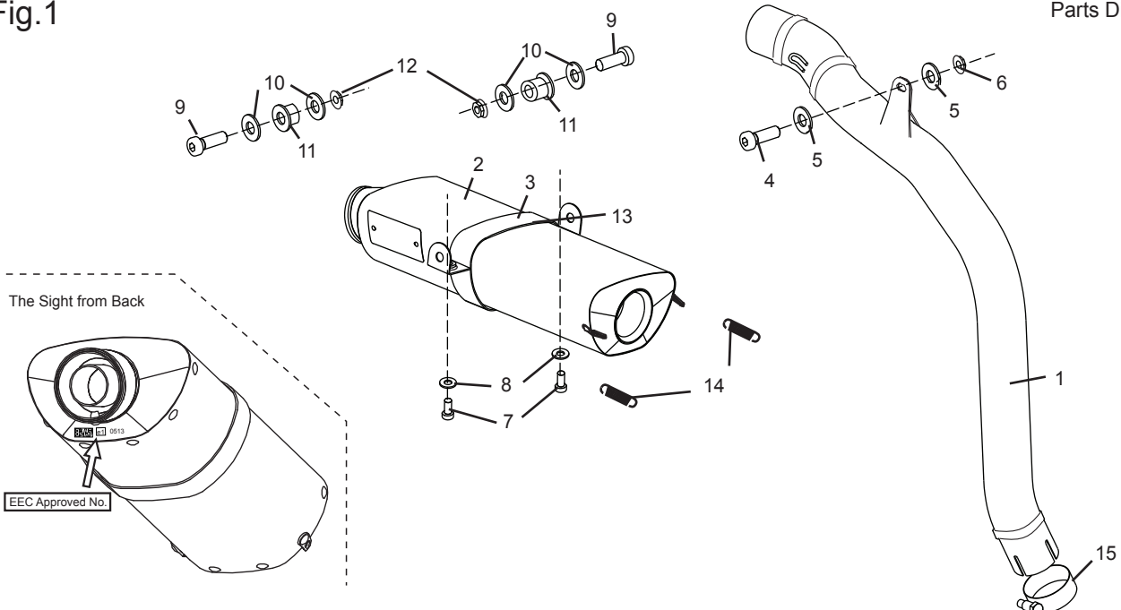
Parts Diagram
